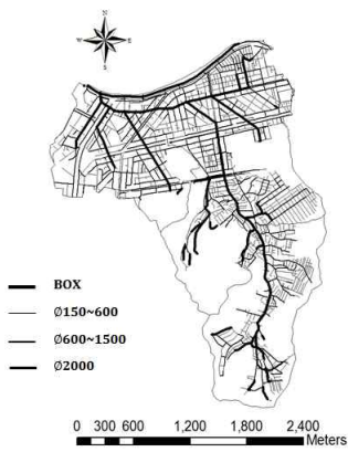
Fig. 5. Storm Sewer of Study area
